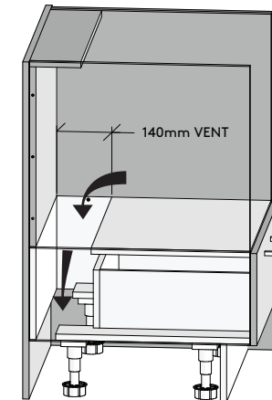
Ventilation: Option 2 140mm × cabinet width vented down into kick panel space
