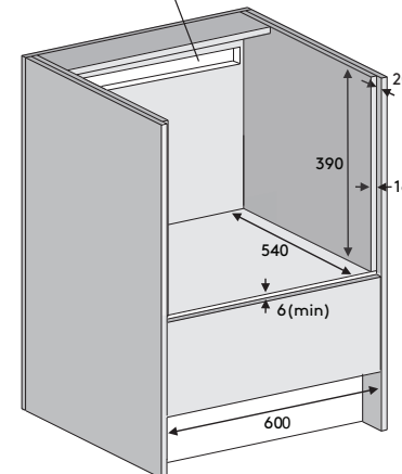
Ventilation: Option 1 Cutout 45mm × 500mm top rear of cabinet
